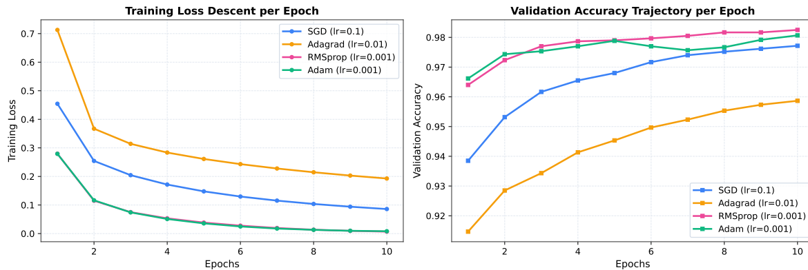
Figure 6: Convergence Rate & Accuracy Across Optimization Algorithms
