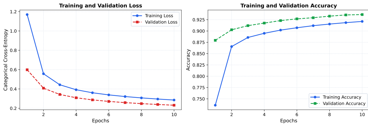
Figure 3: Learning Curves for Baseline DNN (Mini-batch SGD, lr=0.01, Batch=128)
