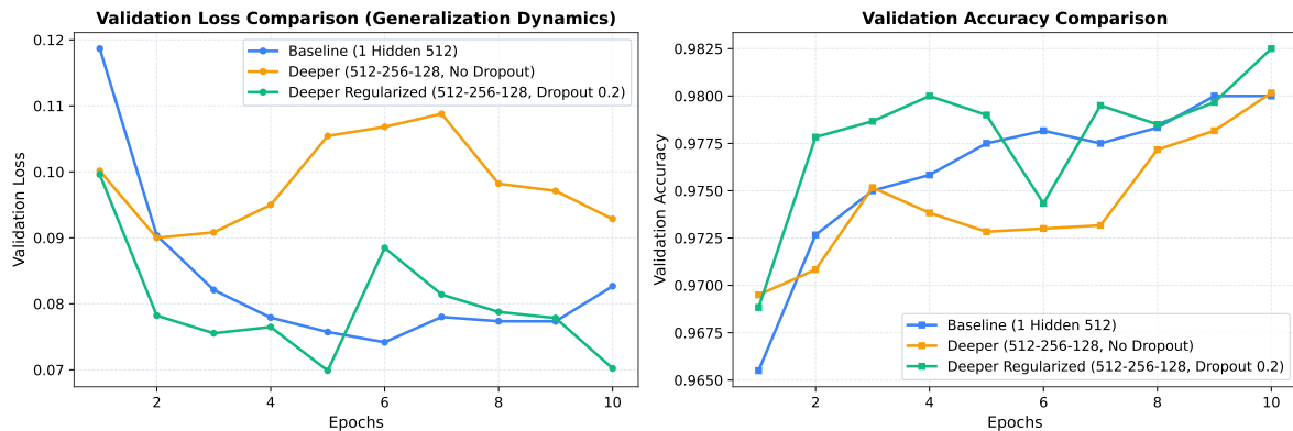
Figure 7: Impact of Architectural Depth & Dropout Regularization on Generalization
