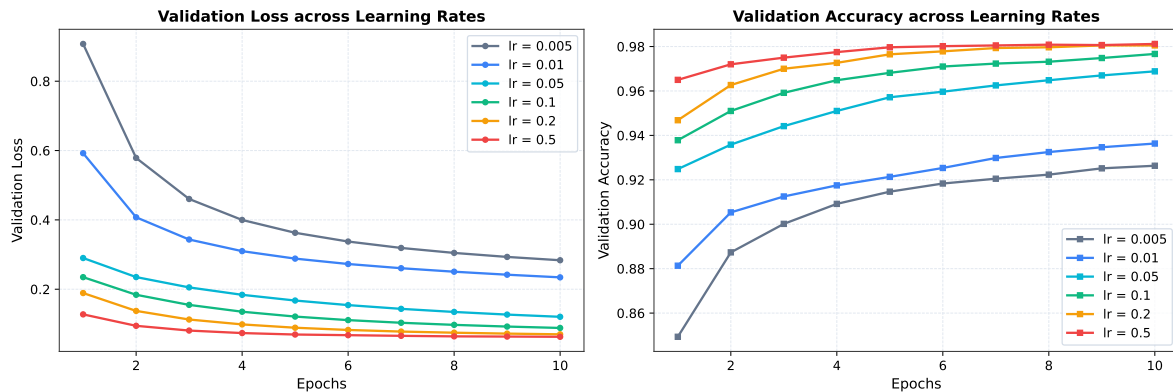
Figure 5: Learning Rate Sensitivity Analysis on Model Convergence (SGD, 10 Epochs)
